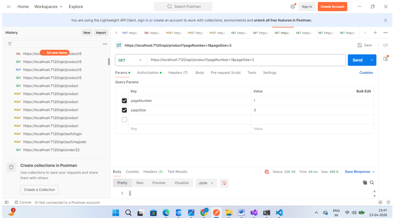
Screenshot 5.1a — Pagination query parameters: pageNumber and pageSize.
