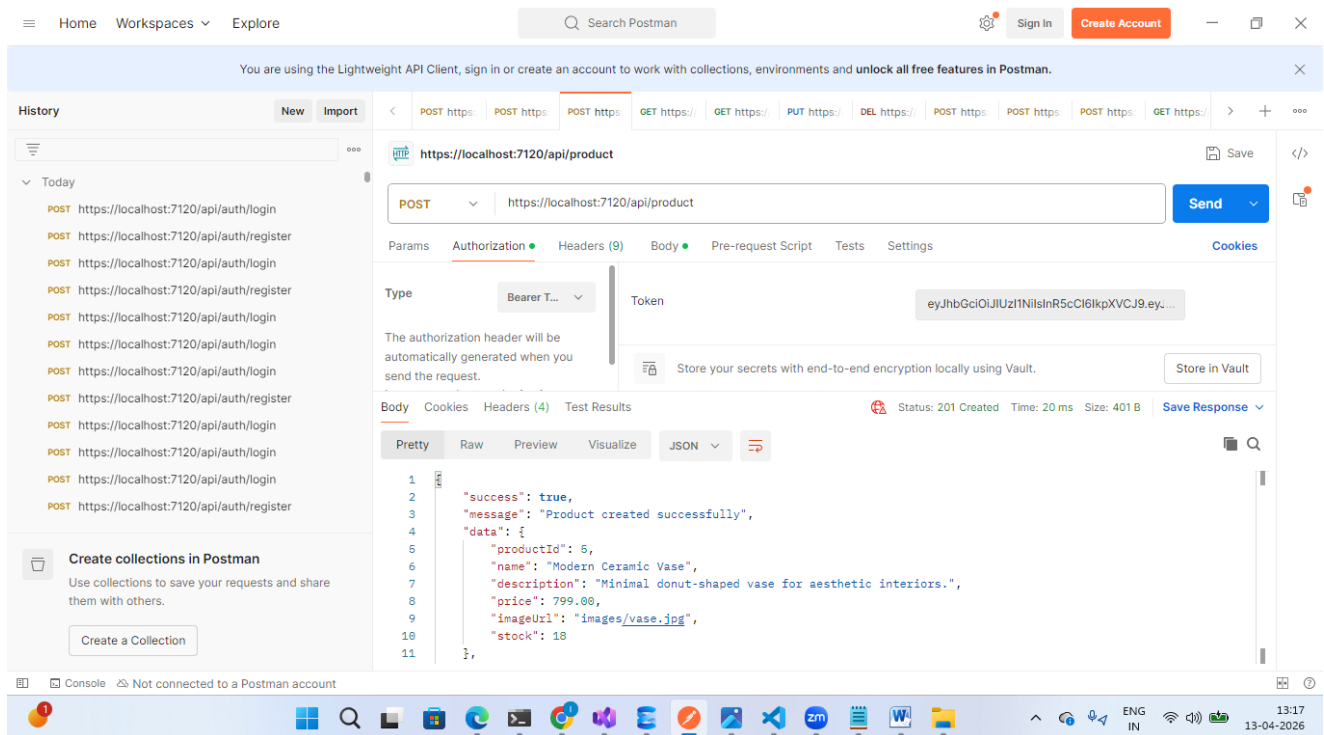
Screenshot 3.1a — Valid admin JWT token added to Authorization header.
