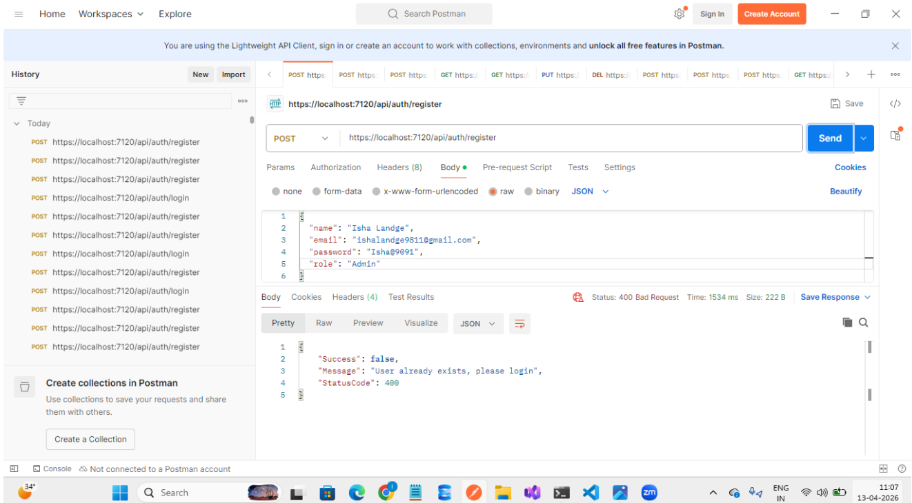
Screenshot 2.1c — Error returned when registering an already-existing user.
