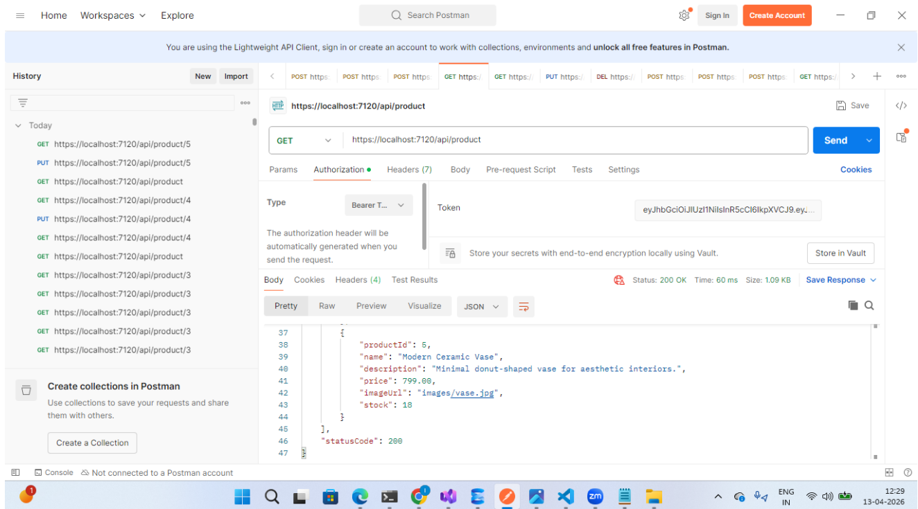
Screenshot 3.3e — Product ID 5 details before update.
