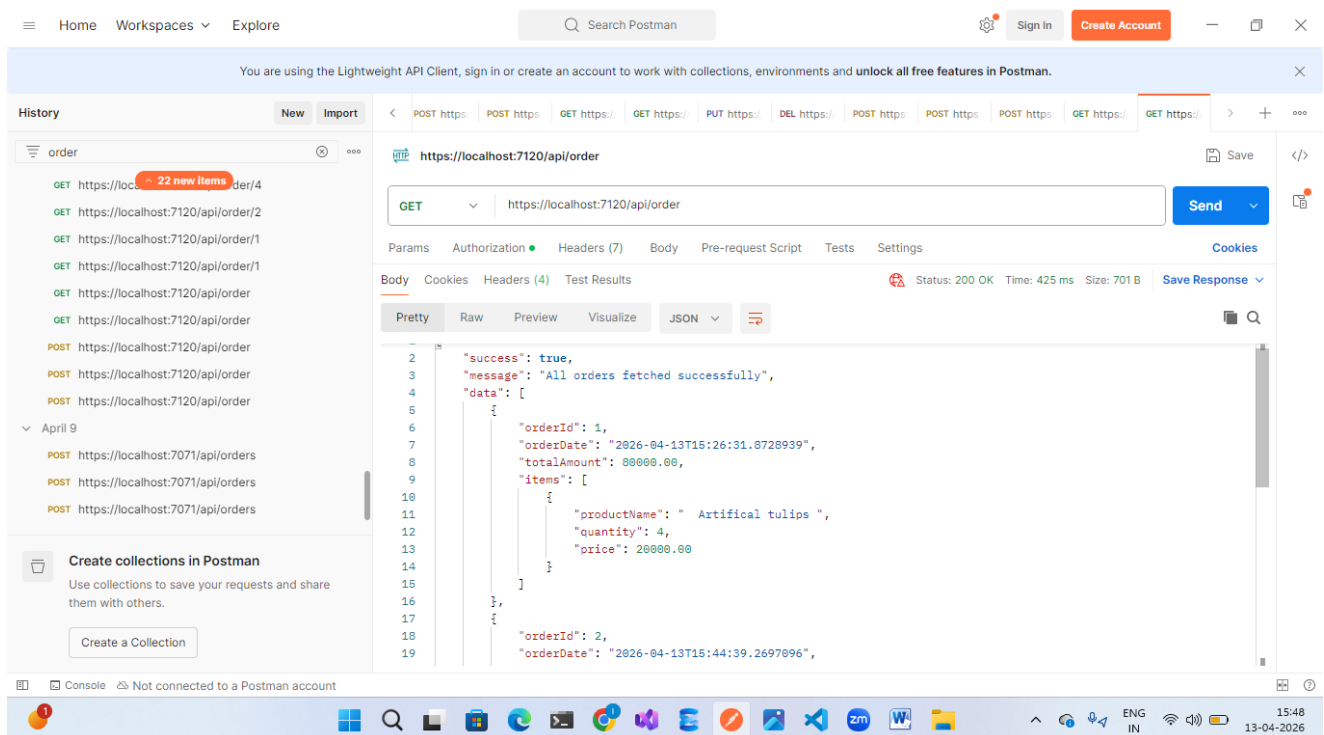
Screenshot 4.2d — Orders list (page 1).
