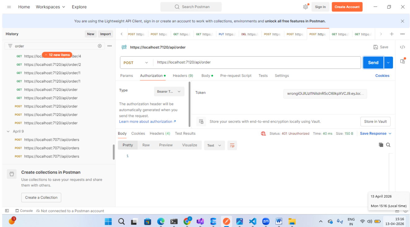
Screenshot 4.1b — Invalid JWT token returns 401 Unauthorized.
