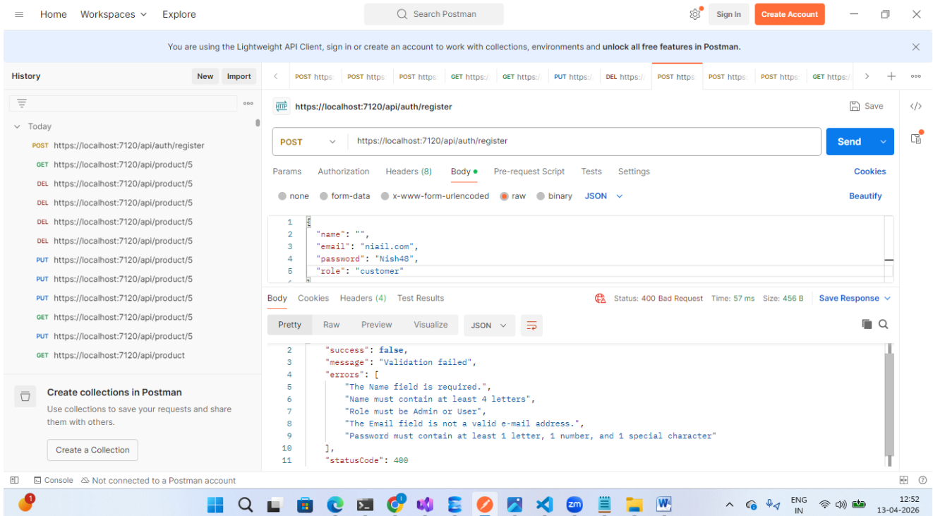
Screenshot 2.3b — Validation error during user registration (missing or invalid fields).
