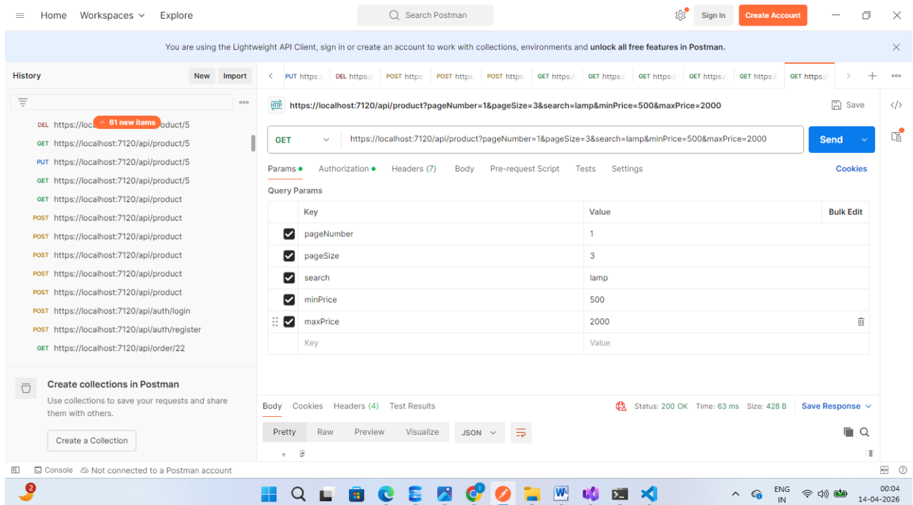
Screenshot 5.4a — Combined query parameters for pagination, search, and price filter.
